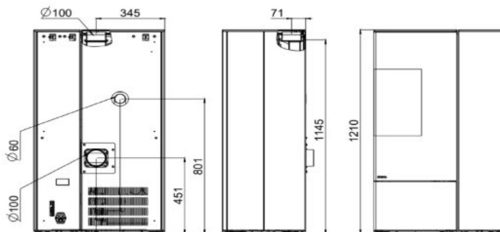
CONNECT PELLET EDGE LINKS E26/E40
